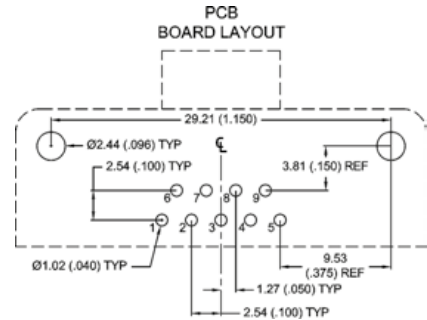
9 CONTACTS - VIEW B
