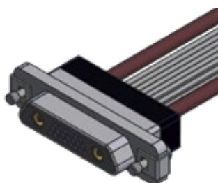
▲ COMBO 51 2 COAX S3 + 21SIGN MALE PIGTAIL (C3)
