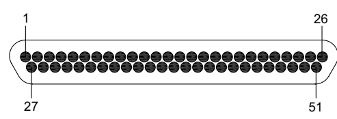
51 CONTACTS DOUBLE ROW (51DR)
